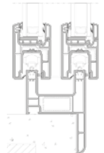
Detail 2 with gasket
