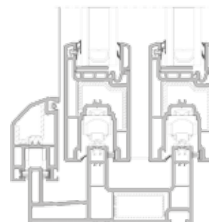
Detail 3 with gasket
