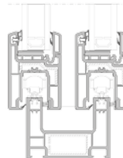
Detail 1 with gasket
