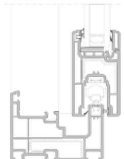
Detail 4 with gasket
